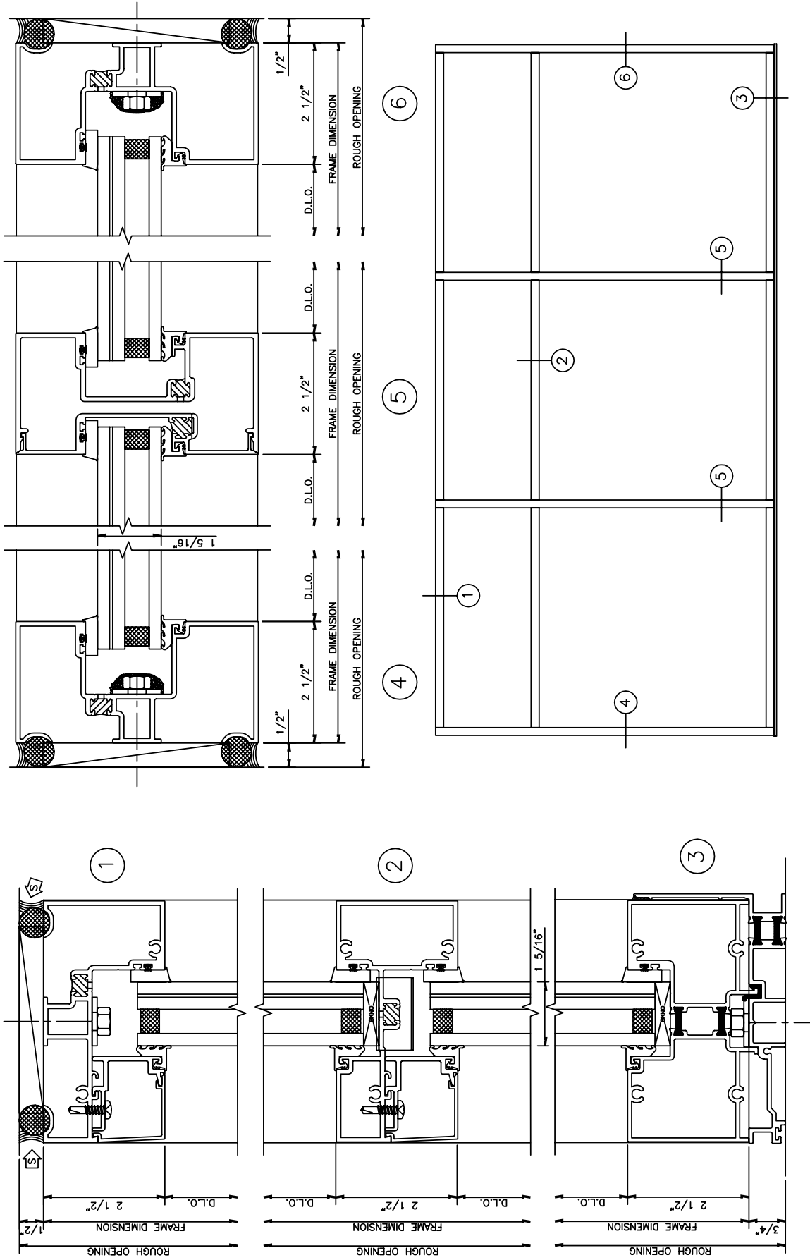
2 1/2" X 5" IMPACT/BLAST GRADE THERMAL IMPACT STOREFRONT FRAME
