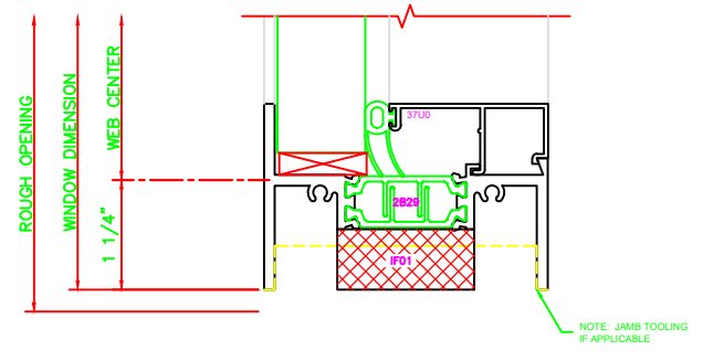
200 SILL 325 FIXED
