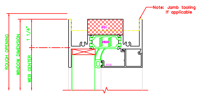
100 HEAD 325 FIXED
